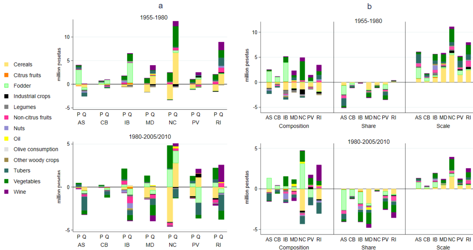
Figure S1. a: Decomposition of the changes into the price and quantity effects (million pesetas). b: Decomposition of the changes into the composition, share and scale effects by region (million pesetas). ‘Other’ regions. AS: Asturias; CB: Cantabria; IB: Balearic Islands; MD: Madrid; NC: Navarra; PV: Basque Country; and RI: La Rioja. Source: Own elaboration from MAPAMA (1955, 1980, 2005, 2010).
