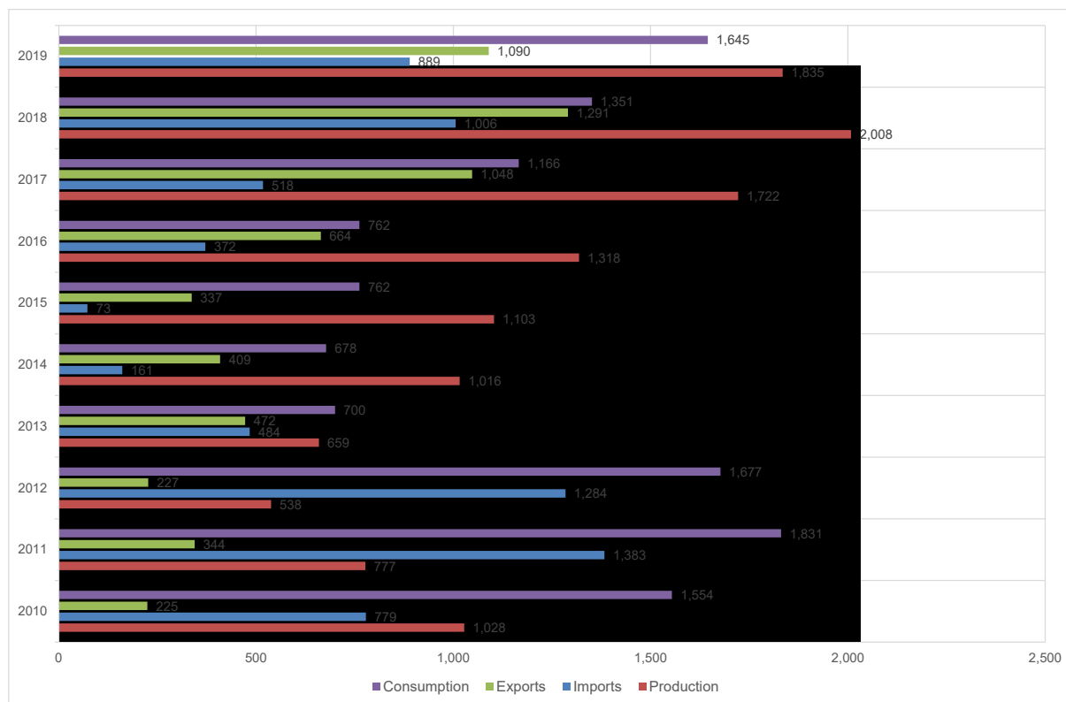
Figure S1. Spanish biodiesel gross inland consumption, production, imports, and exports ( \times 1000 \text{ m}^3 ). Source: CNMC (2019a).
