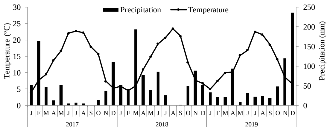
Figure S1. Average monthly temperature and precipitation during the experimental period in the weather station of Sta Apolónia Farm in Bragança.
