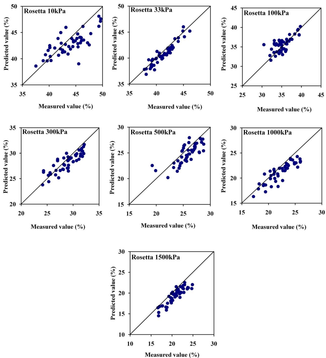
Supplementary Figure S3. The scatter plots of the measured vs. predicted water content for testing data using Rosetta model.
