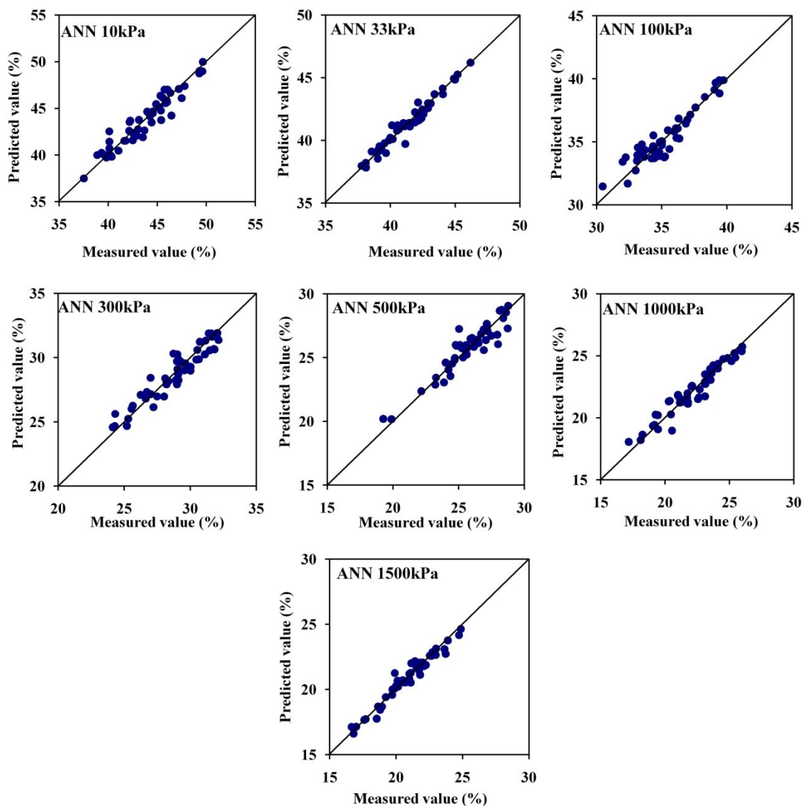
Supplementary Figure S4. The scatter plots of the measured vs. predicted water content for testing data using artificial neural network (ANN) model
