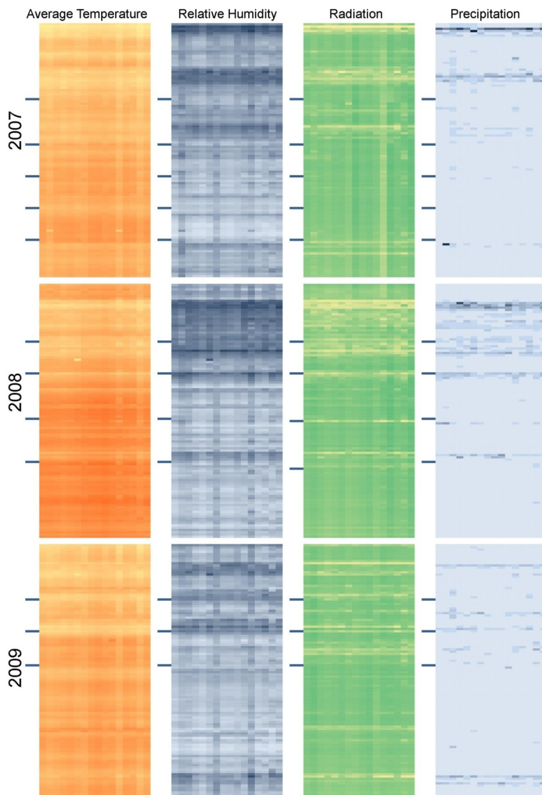
Figure S1. Color-scale representation of meteorological data between 01 May and 20 August 2007, 2008, and 2009, related to the average temperature ( ^{\circ}\text{C} ), relative humidity (%), radiation ( \text{MJ}/\text{m}^2 ), and precipitation (mm).
